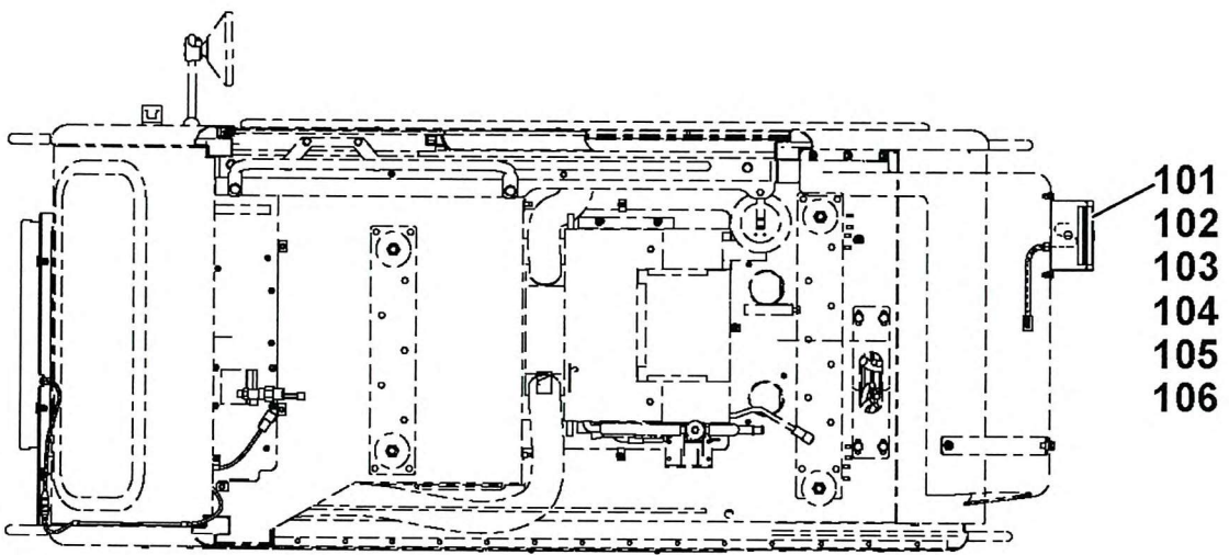
VIEW B-B BOTTOM VIEW
